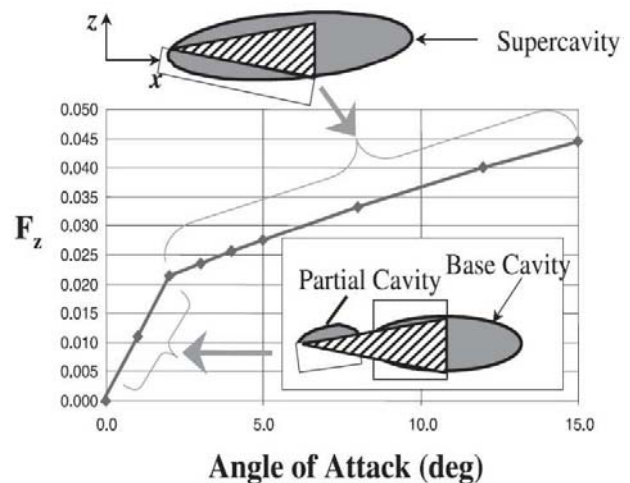
Fig. 3 Variation of fin force. Source : Kirshner [10]
