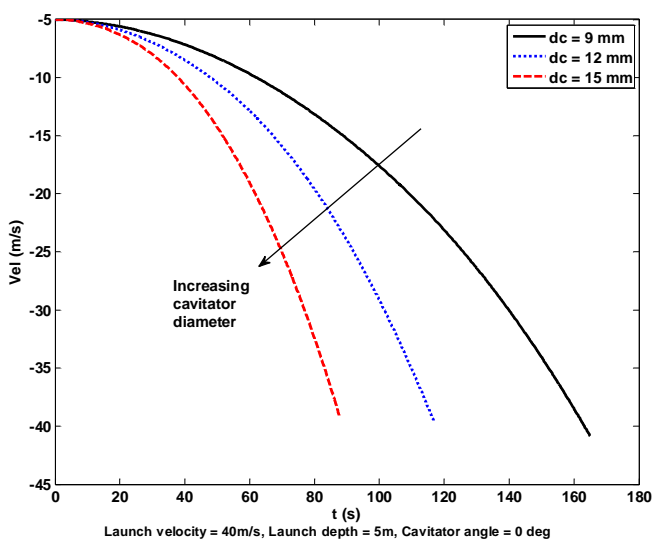
Fig. 11 Trajectory variation with cavitator diameter
