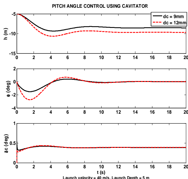
Fig. 14 Pitch angle control using cavimator
