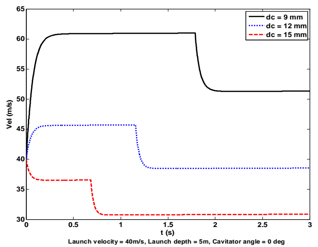
Fig. 12 Velocity variation with cavitator diameter
