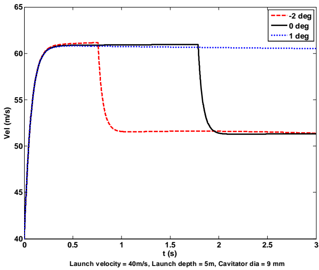
Fig. 10 Effect of cavitator angle on velocity
