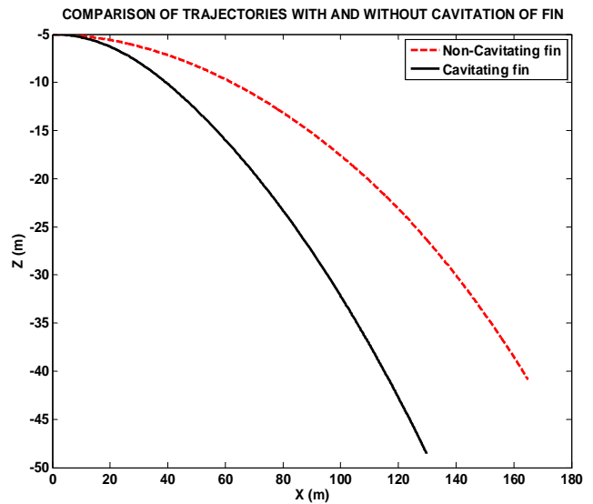
Fig. 8 Variation in trajectory due to fin cavitation
