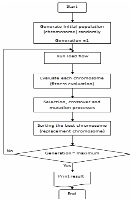
Fig. 2 Flow of optimal allocation of EG using RCGA
