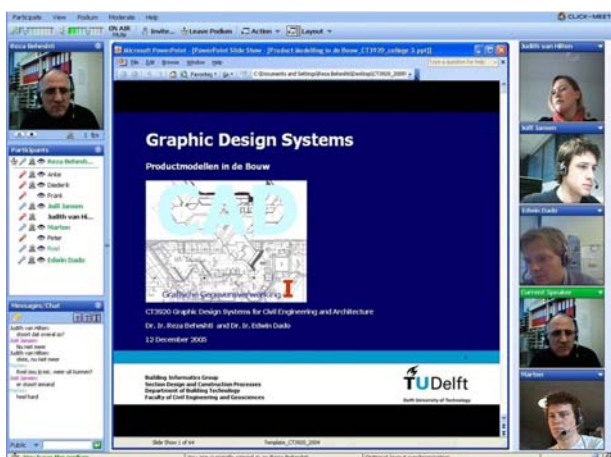
Fig. 8 Virtual classroom
