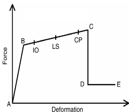
Fig. 9 Force-deformation relationship of typical Plastic hinges
