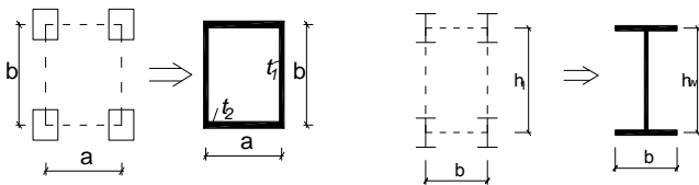
Fig. 4 Equivalent model of column and beam
