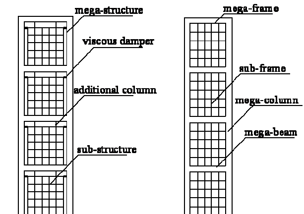
Fig. 2 MSCSS configuration
