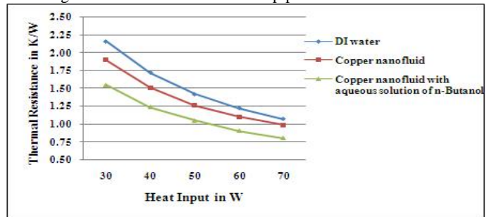
Fig.13 Thermal resistance of heat pipe for 90° inclination
