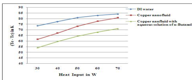
Fig 14 Variation of (T_e - T_c) for 0^\circ inclination
