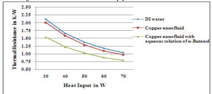
Fig.11 Thermal resistance of heat pipe for 60° inclination
