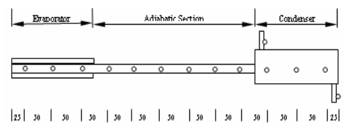
Fig. 1(b) Thermocouple locations of heat pipe
