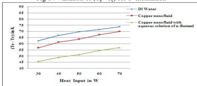
Fig 15 Variation of (T_e - T_c) for 15^\circ inclination
