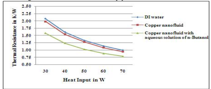
Fig.10 Thermal resistance of heat pipe for 45° inclination
