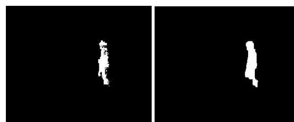
(a) without gradient model (b) with gradient model Fig. 6 Foreground image obtained with gradient
