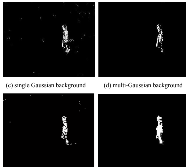
(c) single Gaussian background (d) multi-Gaussian background (e) Non-parametric background (f) parametric background Fig. 5 Methods comparison for foreground detection
