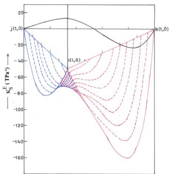
Fig. 4 Excess isentropic compressibilities, \kappa_S^E for 2-pyrrolidinone (i) + toluene (j) + ethanol (k) ternary mixture at 308.15 K
