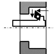
(b) Internal Step Turning Fig. 23 Processes in Process Plan 2
