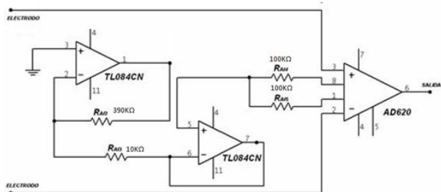
Fig. 5 Amplifier circuit
