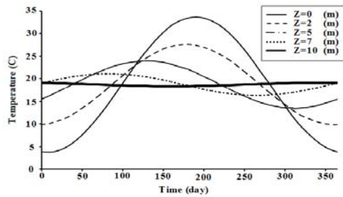
Fig. 2 Ground temperature profile at different depth
