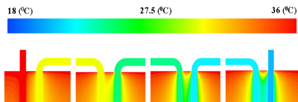
Fig. 7 Contour of temperature around each borehole
