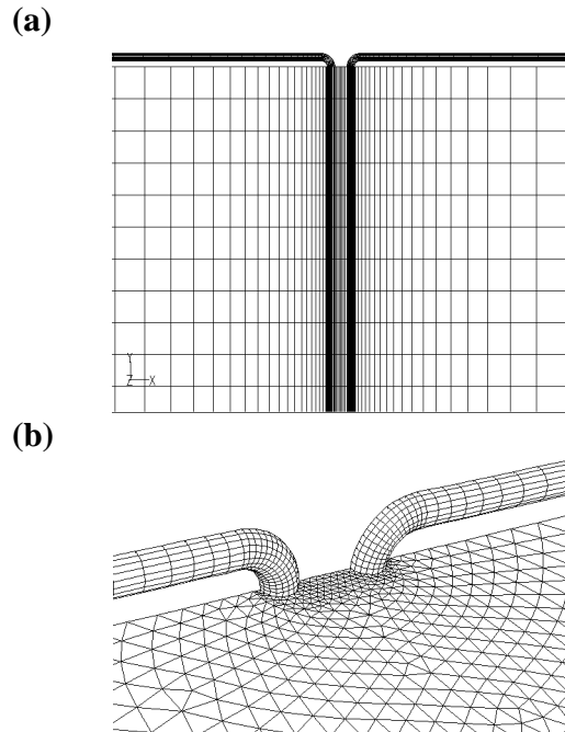
Fig.4 (a) Schematic of the computational grid in the symmetry plane of one borehole (b) Magnification of mesh neighboring to one borehole
