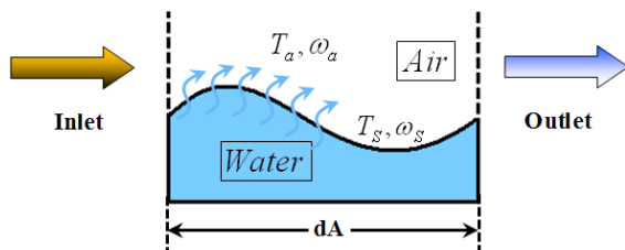
Fig. 6 Schematic of direct evaporation process
