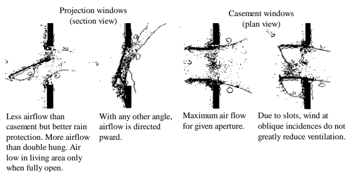
Fig. 1 Airflow patterns through windows
