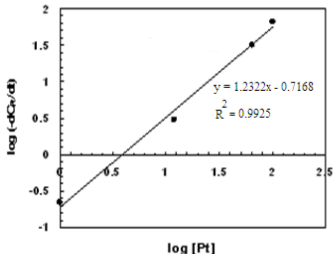
Fig. 7. A plot of \log (-dC_{Pt}/dt) vs. \log [Pt] . Determining n value so as to determine k value of platinum using Differential Method of Data Analysis at ambient conditions. [Na_2S_2O_3] = 0.05 M and HCl = 1 M].
