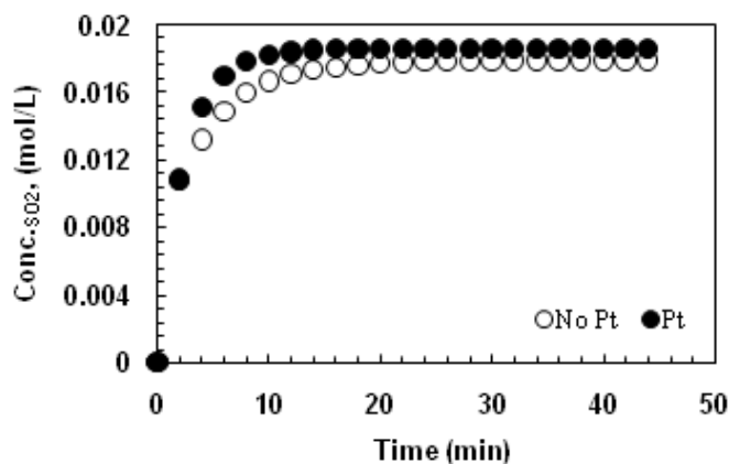
Fig. 15. A plot of SO_2 concentration vs. mixing time. Reactive absorption of SO_2 in solution with or without Pt ions. [HCl] = 4 M .
