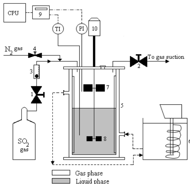
Fig. 2. Stirred cell reactor: SO_2 gas inlet and outlet valves (1, 2); SO_2 gas flowmeter (3); N_2 gas inlet valve (4); stirred cell reactor (5); thermostat water bath (6); gas stirrer (7); liquid stirrer (8); data logger (9); magnetic coupling mixer (10).
