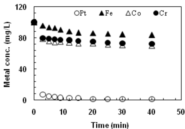
Fig. 5. A plot of metal concentration vs. contact time. Precipitation kinetics of platinum and base metals from a mixed solution in liquid-liquid batch test at ambient conditions, [ Na_2S_2O_3 ] = 0.05 M and [ HCl ] = 1 M].
