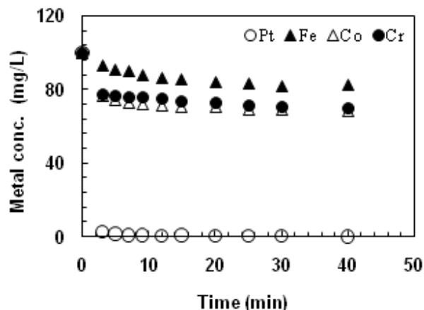
Fig. 3. A plot of metal concentration vs. contact time. Precipitation kinetics of platinum and base metals from a mixed solution in liquid-liquid batch test at ambient conditions, [ HCl ] = 1 M, [ Na_2S_2O_3 ] = 1 M].
