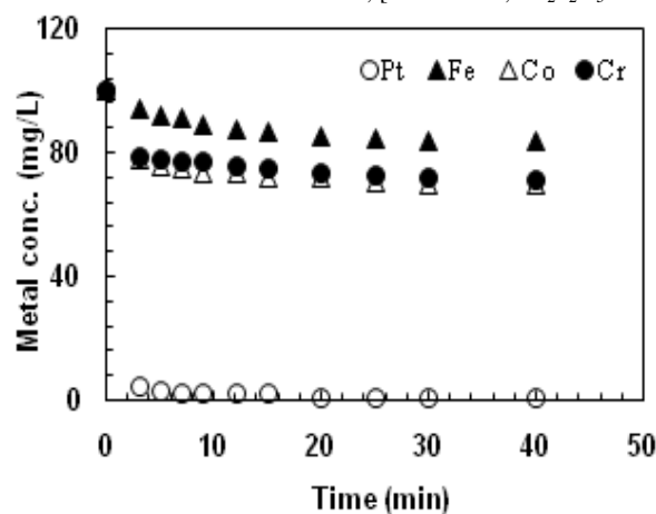
Fig. 4. A plot of metal concentration vs. contact time. Precipitation kinetics of platinum and base metals from a mixed solution in liquid-liquid batch test at ambient conditions, [ Na_2S_2O_3 ] = 0.1 M and [ HCl ] = 1 M].
