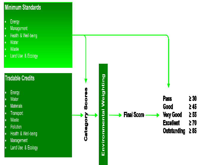
Fig. 1 General BREEAM process
