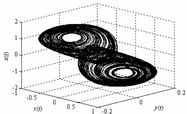
Fig. 1 The modified Chua's circuit chaotic attractor
