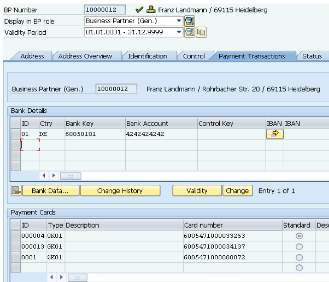
Fig. 2 SAP business partner containing collections of objects
