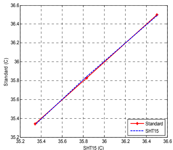
Fig. 10 Relative humidity measurement calibration
