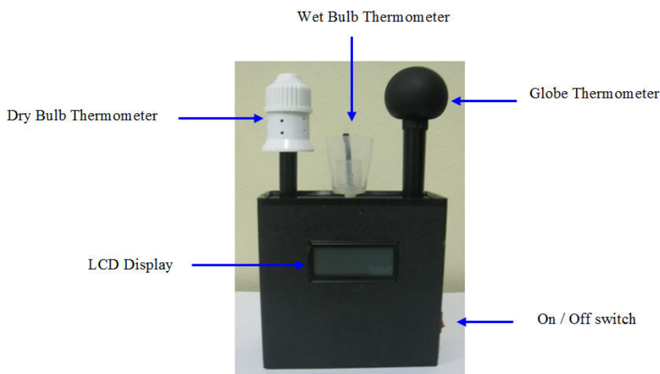
Fig. 2 Heat stress monitor device
