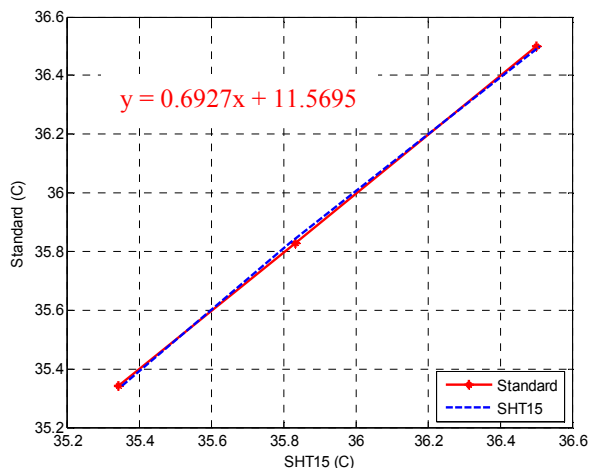
Fig. 8 Dry bulb temperature measurement calibration
