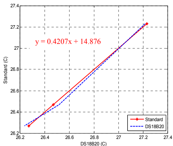
Fig. 9 Wet temperature measurement calibration
