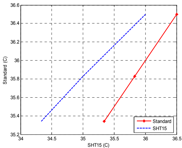
Fig. 4 Dry bulb temperature measurement
