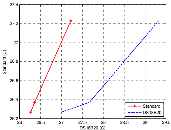
Fig. 5 Wet temperature measurement
