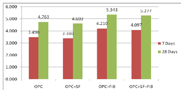
Fig.13 Flexural Strength for Prism Specimens (in N/mm^2 )
