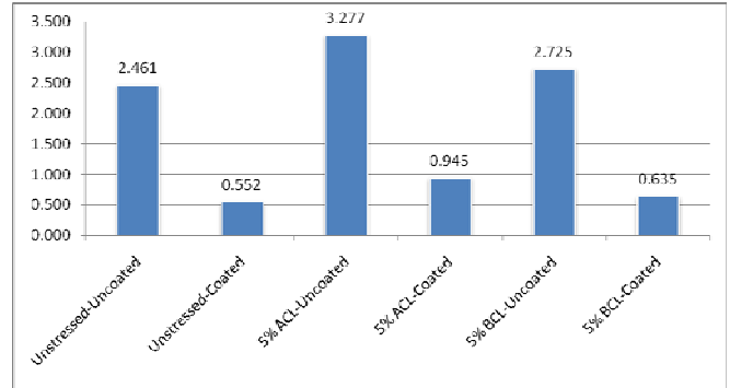
Fig.11 Weight loss of rebars for specimens of OPC+SF+Fibre (in %)
