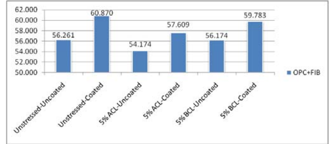
Fig. 6 Load Carrying Capacity for Specimens of OPC+Fibre (in kN)
