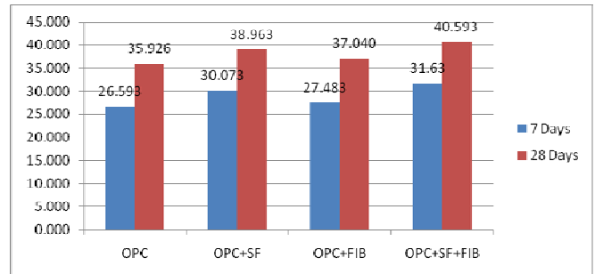
Fig. 12 Compressive Strength for Cube Specimens (in N/mm 2 )
