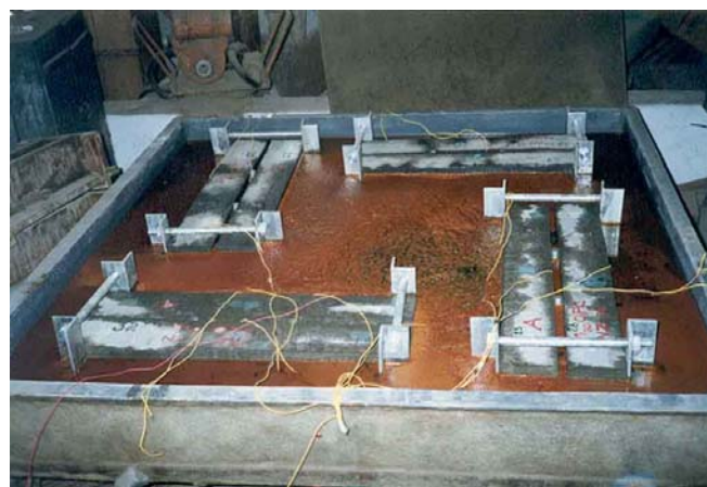
Fig. 2 Accelerated Corrosion process for stressed Condition
