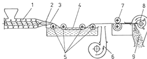
Fig. 1 Compounding process principle
