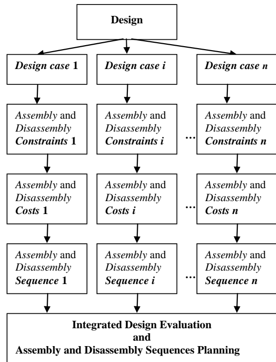
Fig. 2 The flow of the integrated design evaluation and assembly and disassembly sequence planning
