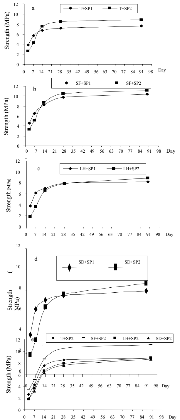
Fig. 3 Tensile strength (MPa) of the studied RPC [2]
