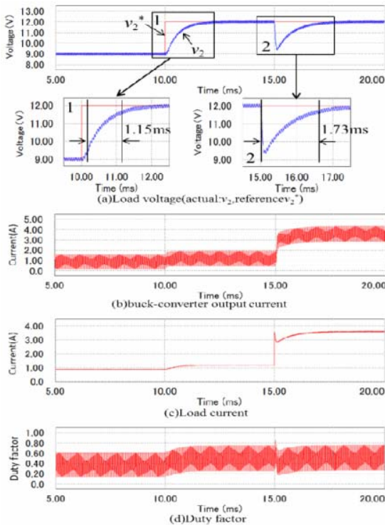
Fig. 8 Conventional ILQ control by 2 nd -order polynomial \alpha_1=5000^2, \alpha_2=2*1*5000, \sigma=40000, G_f(s)=1 and G_R(s)=0
