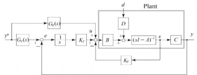
Fig. 3 Block diagram of the 2D-ILQ servo-system
