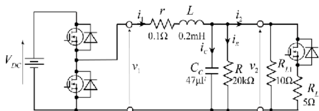
Fig. 1 The buck-converter circuit
