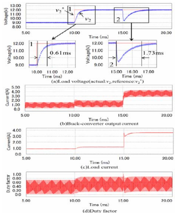
Fig. 12 Responses to 100% error of L in Fig. 10
