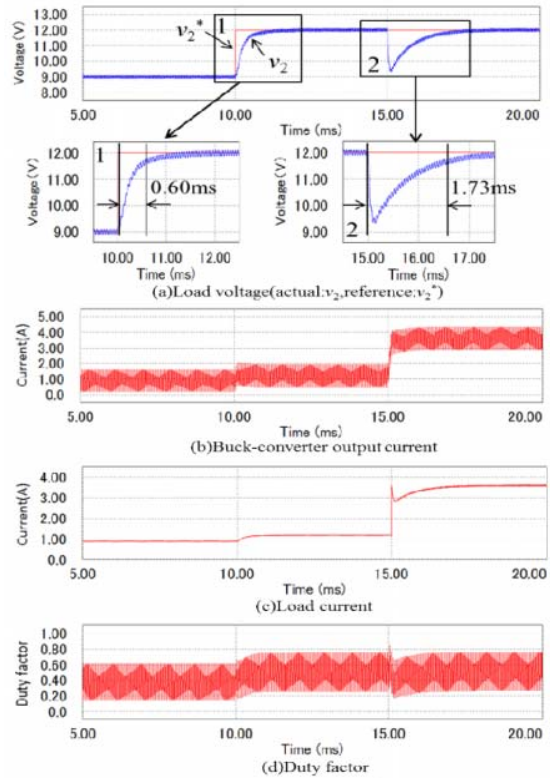
Fig. 10 Proposed 2D-ILQ control by 2 nd -order polynomial \alpha_1=5000^2, \alpha_2=2*1*5000, \sigma=40000,
