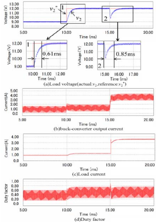
Fig. 9 Conventional ILQ control by 2 nd -order polynomial \alpha_1=7500^2, \alpha_2=2*1*7500, \sigma=40000, G_f(s)=1 and G_R(s)=0
