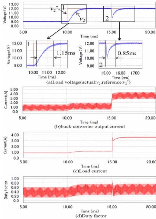
Fig. 11 Proposed 2D-ILQ control by 2 nd -order polynomial \alpha_1=7500^2, \alpha_2=2*1*7500, \sigma=40000, G_F(s) = \frac{2500}{s+2500} and G_R(s)=0
