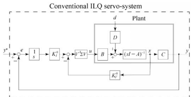
Fig. 4 Block diagram of the 2D-ILQ servo-system with G_F(s)=1 and G_R(s)=0
