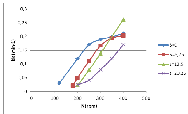
Fig. 11 k_L a for different submersions
