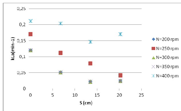
Fig. 12 k_L a for different rotational speed
