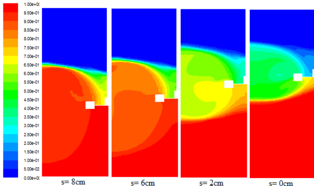
Fig. 5 Contours of phases for different submergences
