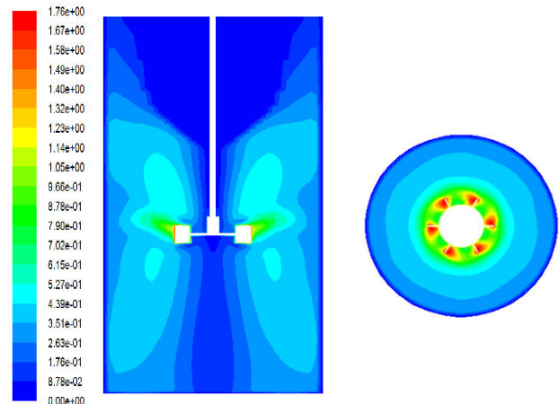
Fig. 4 Contours of global velocity
