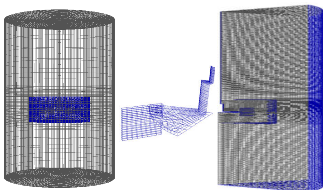
Fig. 2 Mesh of the studied field
