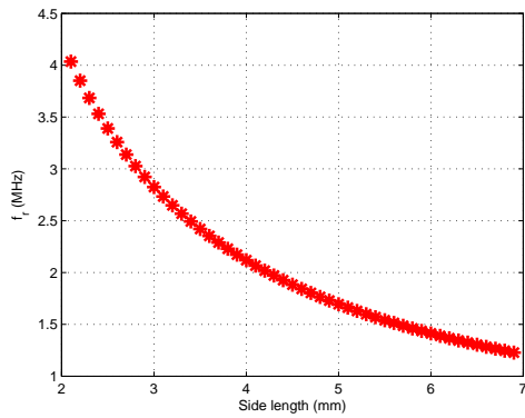
Fig. 5 Resonance frequency versus transducer side length calculated for a piezoelectric layer thickness of 1 \mu\text{m}
