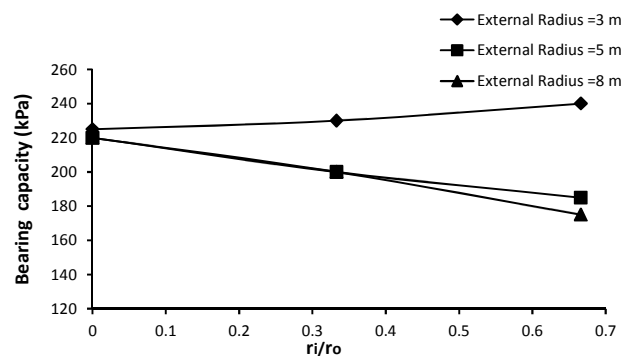
Fig. 4 Bearing capacity changes with increase in r_i/r_o ratio when clay layer thickness is 9 (m)
