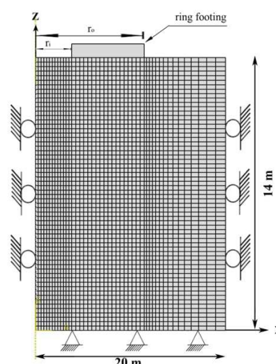
Fig. 1 Grid of axis-symmetric model and boundary conditions
