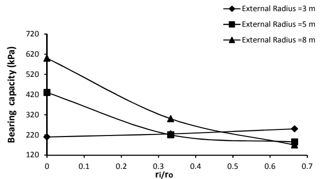
Fig. 2 Bearing capacity changes with increase in r_i/r_o ratio when clay layer thickness is 2 (m)
