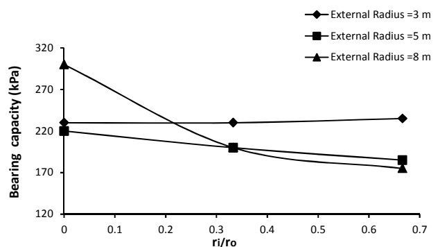
Fig. 3 Bearing capacity changes with increase in r_i/r_o ratio when clay layer thickness is 5 (m)
