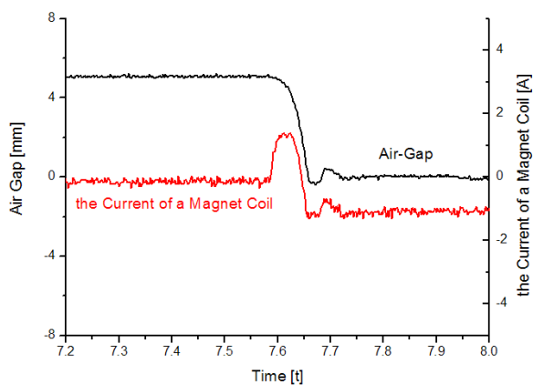
Fig. 12 An air-gap and magnet coil current for the step-down motion of the position
