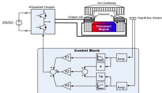
Fig. 1 Block Diagram of the Levitation Control System
