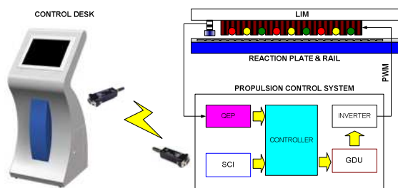
Fig. 8 Block Diagram for propulsion system
