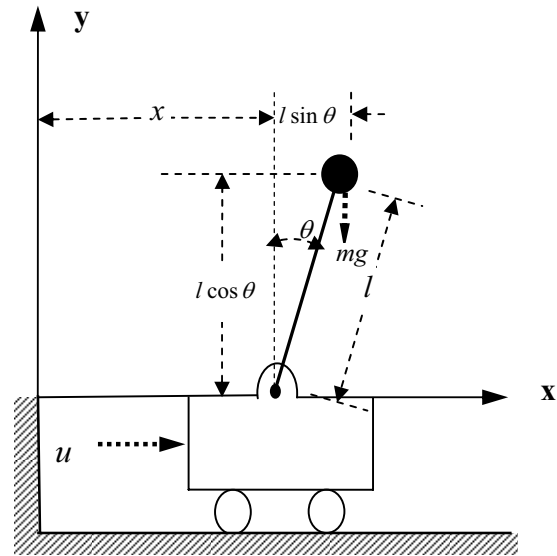
Fig. 1 Schematic model of SIPMC
