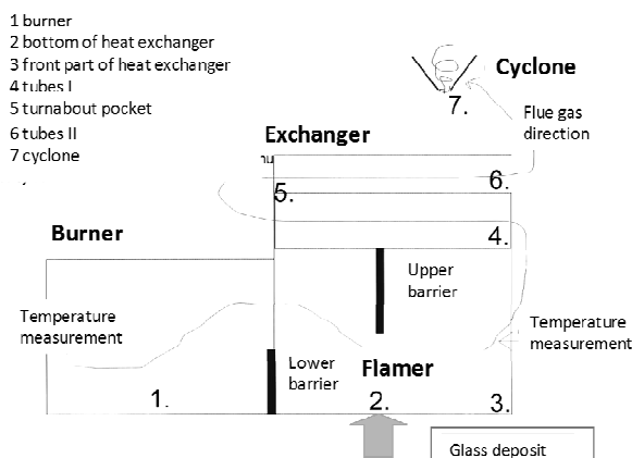
Fig. 2 Locations in a boiler from where samples were collected
