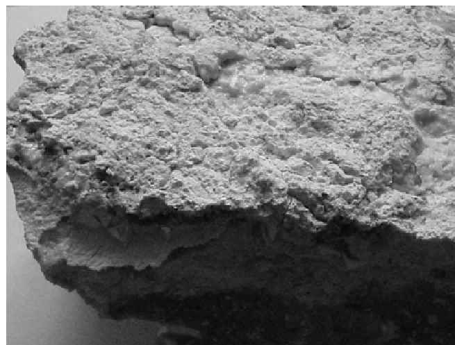
Fig. 1 Glass deposit removed with a layer of refractory ceramics
