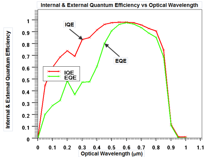
Fig. 5 Internal and external quantum efficiency versus optical wavelength of the single junction Al_xGa_{1-x}As/GaAs solar cell when x varies from 0.85 to 0
