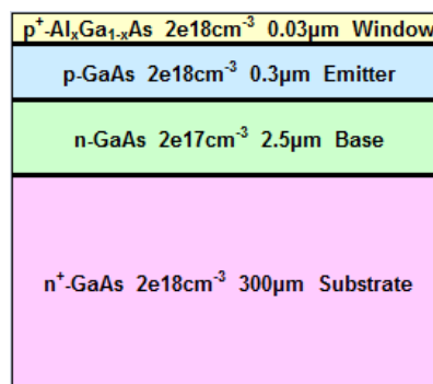
Fig. 1 Structure of the single junction \text{Al}_x\text{Ga}_{1-x}\text{As}/\text{GaAs} solar cell
