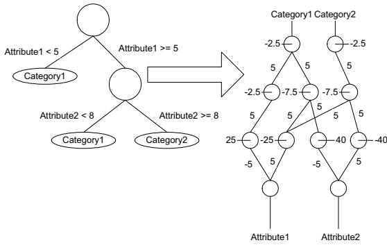
Figure 1. Transformation of decision tree to neural network
