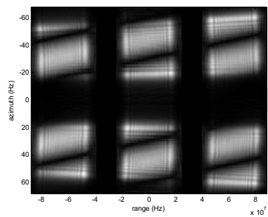
Fig. 4 spectrum with aperture gaps and band gaps
