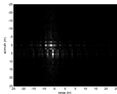
Fig. 5 Image from sparse spectrum
