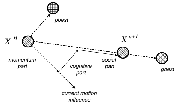
Fig. 1 Position updates in PSO for a two dimensional parameter space.
