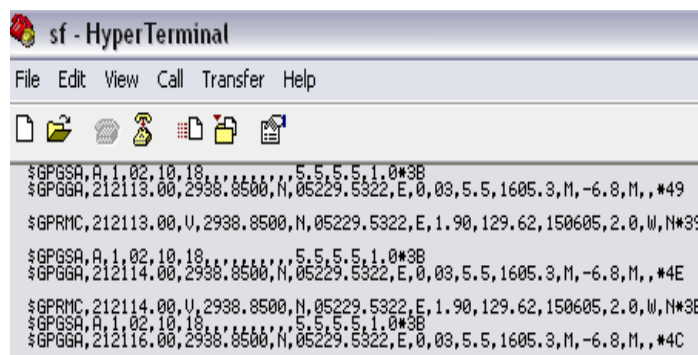
Fig. 2 information has sent by GPS model RFG2k, and shows the information on HyperTerminal software
