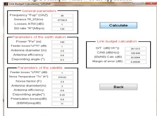
Fig. 3 Calculation of the uplink budget
