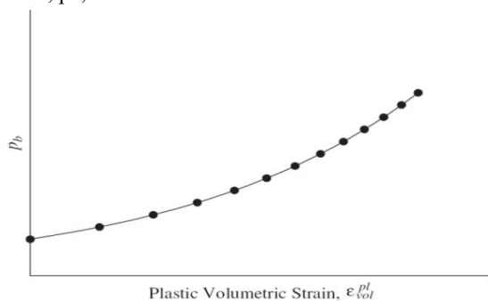
Fig. 3 Typical cap hardening behavior [10]
