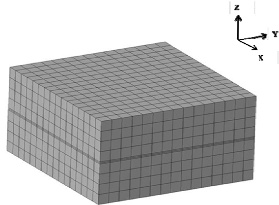
Fig. 6 3D mesh of modeling of direct shear test
