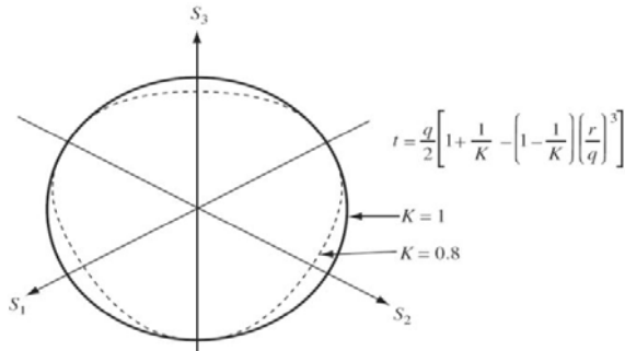
Fig. 2 Projection of the modified cap yield on the-plane [10]
