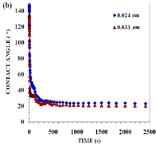
Fig. 2 Relaxation behavior of a) Sn-0.7Cu b) SAC0307 solder on substrate surface
