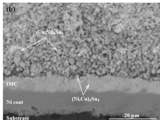
Fig. 4 SEM micrograph of a) Sn-0.7Cu solder/substrate interfacial b) SAC0307 solder/substrate interfacial regions
