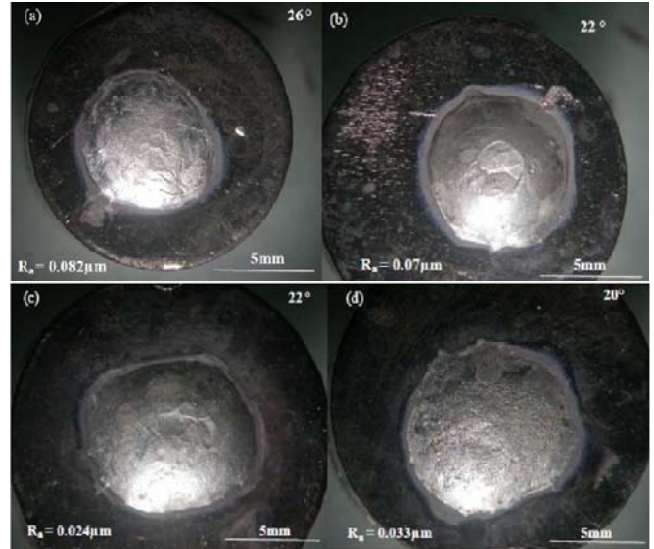
Fig. 3 Macroscopic images (top view) of stabilized alloys on substrate surfaces a – b) Sn-0.7Cu solder and c – d) SAC0307 solder
