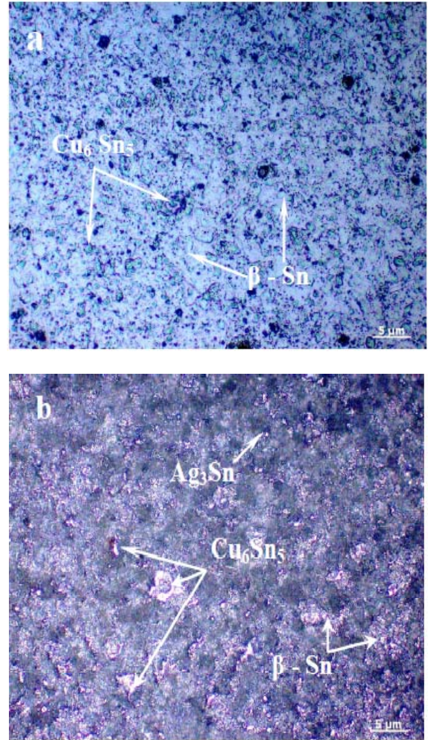
Fig. 1 Optical microstructures of as-received (a) Sn–0.7Cu (b) SAC0307 solder alloys
