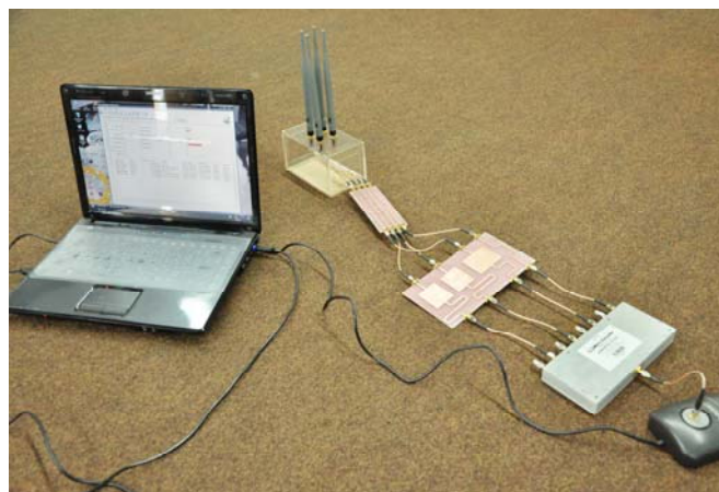
Fig. 6 Measurement setup of proposed system for WMN.
