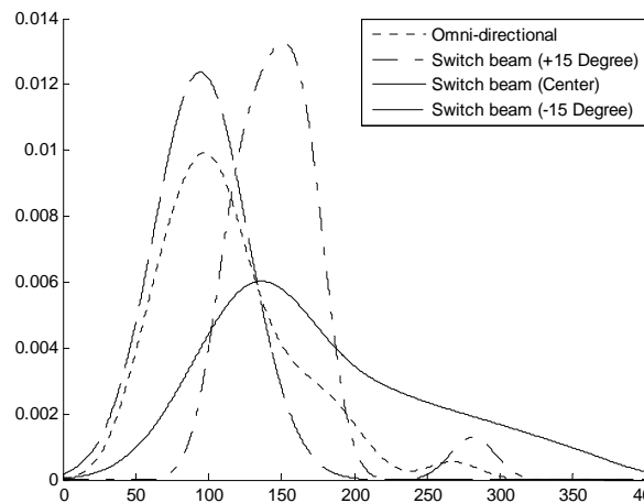
Fig. 11 Probability density function of measured throughput when using conventional omni-directional antenna and proposed switched beam antennas.
