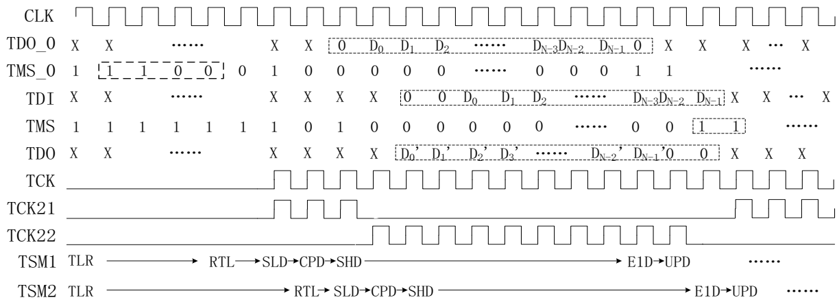
Fig. 10 Timing diagram of this design
