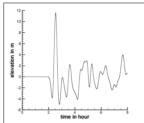
Fig. 6 Computed tsunami response along the coast
