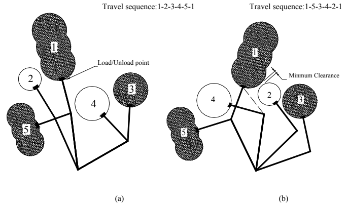
Fig. 3 Machine layout in a robotic cell
