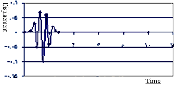
Fig. 3 displacement-time graph (Elsentro earthquake)
