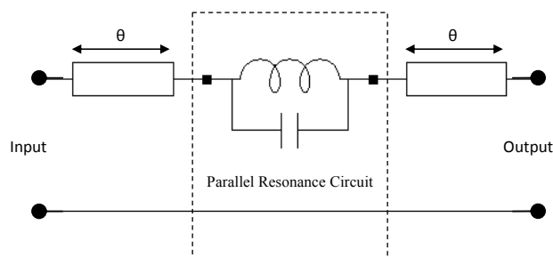
Fig. 9 Basic Equivalent Lumped Circuit Element for the Overall Proposed Structure
