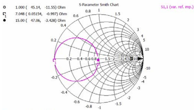
Fig. 10 Smith Chart view of S_{11} of the Meandered Open Circuited Stub using De-embedding Technique
