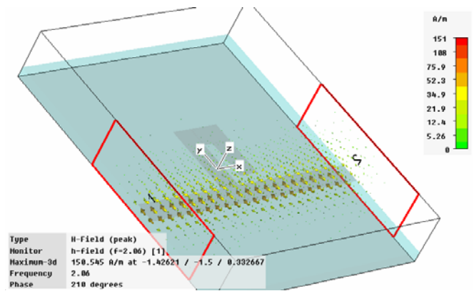
Fig. 4 Vector Plot Magnetic Field Distribution of the Proposed Structure at 2.06 GHz
