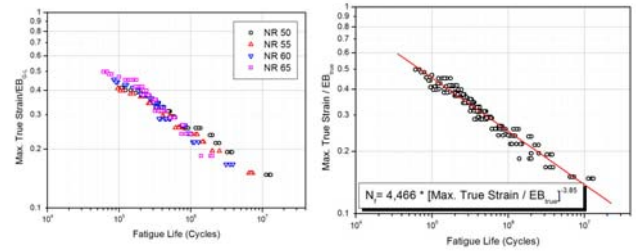
(a) Max. true strain and fatigue life (b) Fatigue life prediction curve
