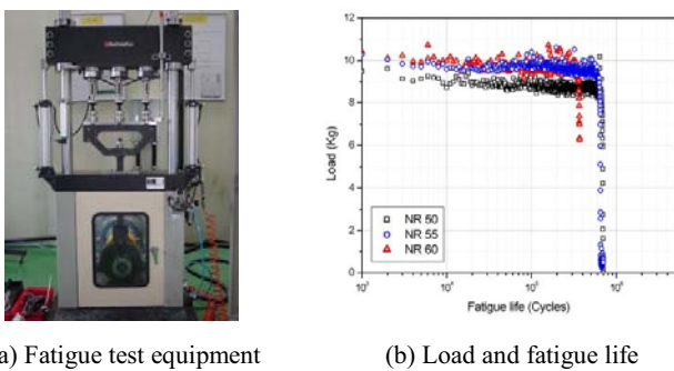
(a) Fatigue test equipment (b) Load and fatigue life Fig. 8 Fatigue test of three-dimensional dumbbell specimen
