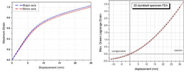
(c) Strain distribution of specimen (d) Displacement and strain curve Fig. 7 Three-dimensional dumbbell specimen for fatigue test
