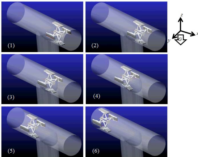
Fig. 8 Simulation results with z-axis gravity
