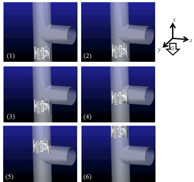
Fig. 7 Simulation results with x-axis gravity
