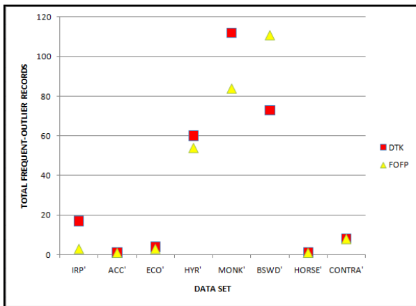
Fig. 5 DTK vs FOFP
