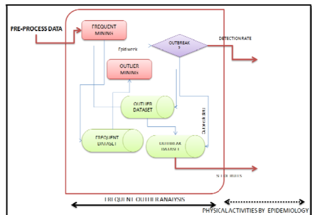
Fig. 2 Anomaly-based Frequent-Outlier (DTK) model
