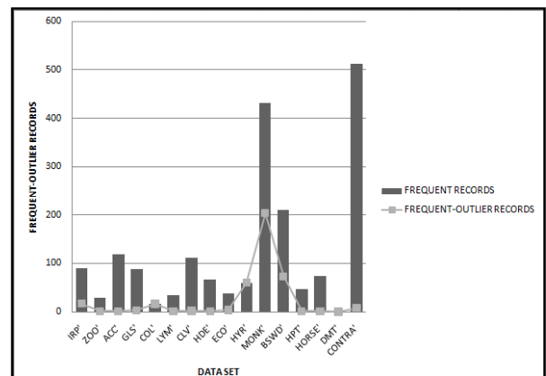
Fig. 4 Outlier records within frequent set records
