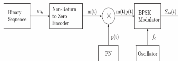
Fig. 2 DS-SS Transmitter block diagram
