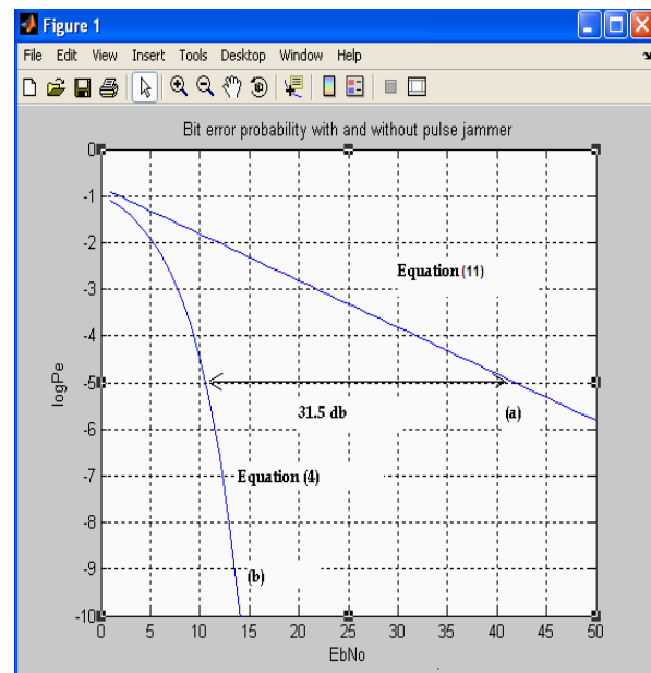
Fig. 4 Bit error probability
