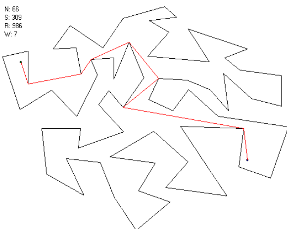
Fig. 4. Example of the algorithm realization.
