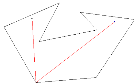
Fig. 1. Minimal link path without using Steiner points
