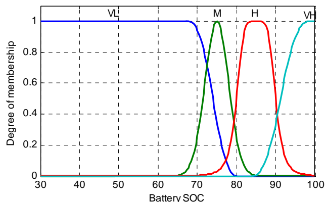
Fig. 2 Membership function plot for Battery SOC
