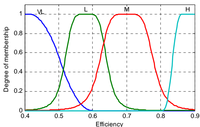
Fig. 3 Membership function plot for Battery Charging Efficiency
