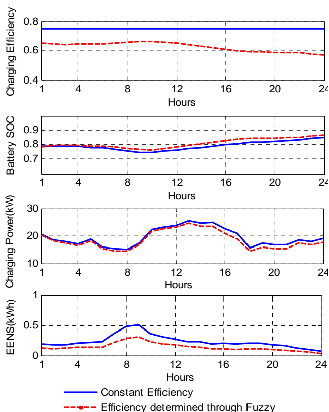
Fig. 6 Effect of Efficiency determined through Fuzzy on parameters of Configuration III
