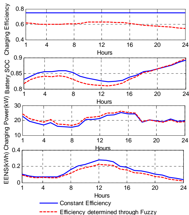
Fig. 4 Effect of Efficiency determined through Fuzzy on parameters of Configuration I
