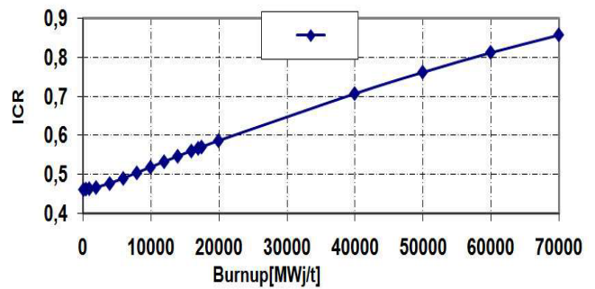
Fig. 15 Index vs. Burnup for Cermet MFE (FBNR)
