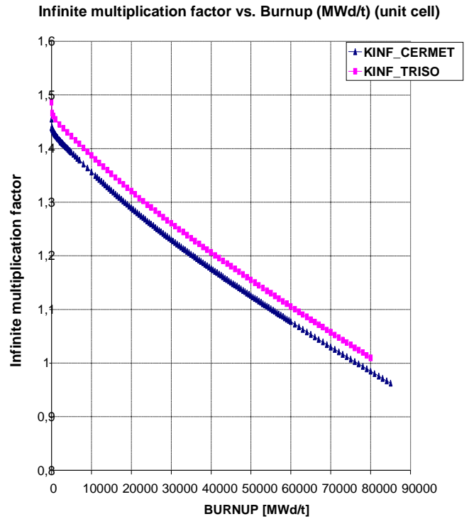
Fig. 9 Infinite multiplication factor vs. Burnup (BWR-PB)
