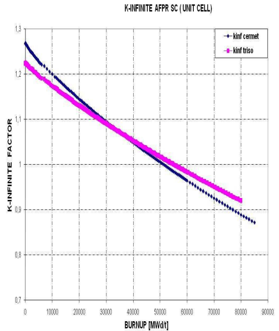
Fig. 6 Infinite multiplication factor vs. Burnup for Cermet and Triso (AFPR-SC)
