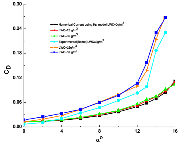
Fig. 4: CD VS AOA for Different Rain rates using K-\epsilon Turbulence Model
