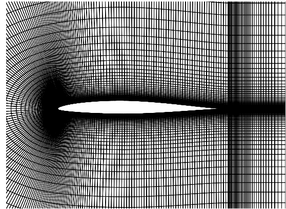
Fig. 1 Grid around Airfoil NACA 64210
