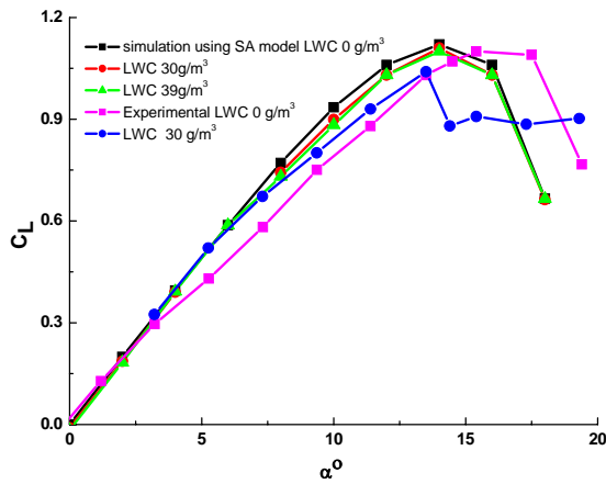
Fig. 10: CL vs. AOA using SA Turbulence Model
