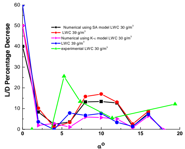
Fig. 13: L/D Percentage Degradation vs. AOA
