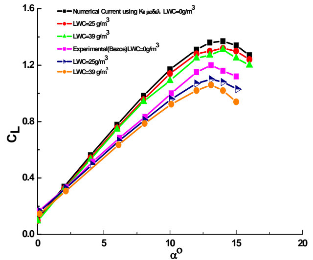
Fig. 5: CL VS AOA using K-\epsilon Turbulence Model
