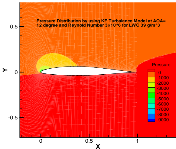
Fig. 16: Pressure Distribution around NACA 64210 LWC 39 g/m 3
