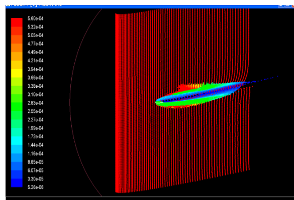
Fig. 14: Particles Tracks around NACA 0012
