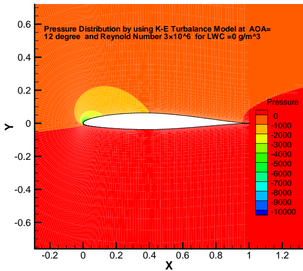
Fig. 15: Pressure Distribution around NACA 64210 LWC 0 g/m 3
