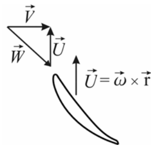
Fig. 2 Schematic diagram for relative velocity formulation
