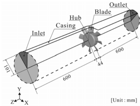
Fig. 3 Solution domain
